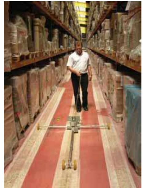
A Concrete Grinding operative using a profileograph to measure floor flatness.
